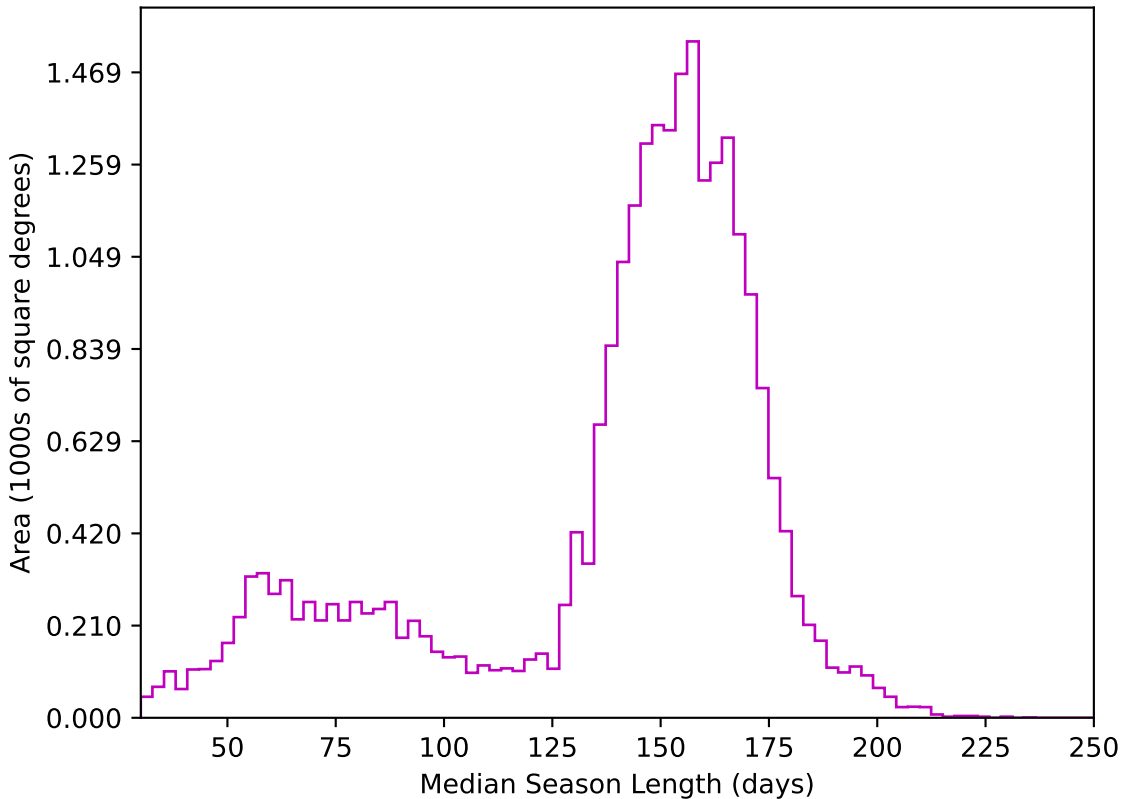
noroll_mjdp270_v3.4_10yrs All sky z band: Median Season Length
