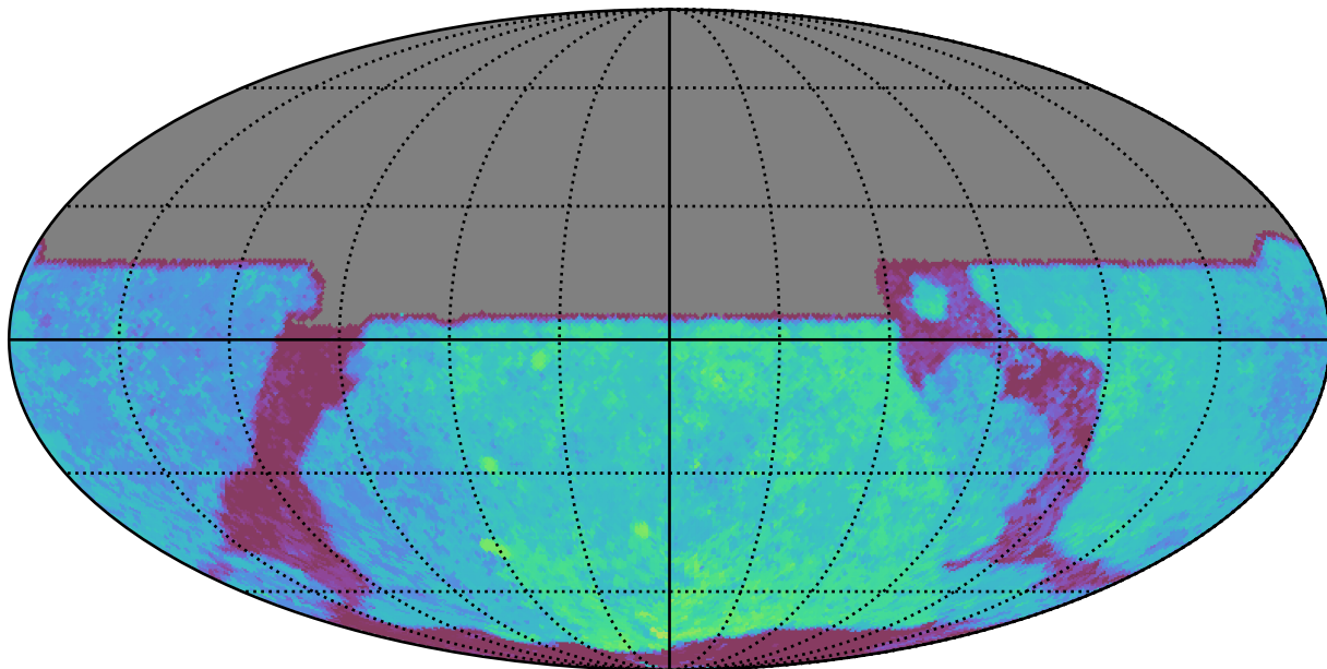
noroll_mjdp270_v3.4_10yrs All sky y band: Median Season Length
