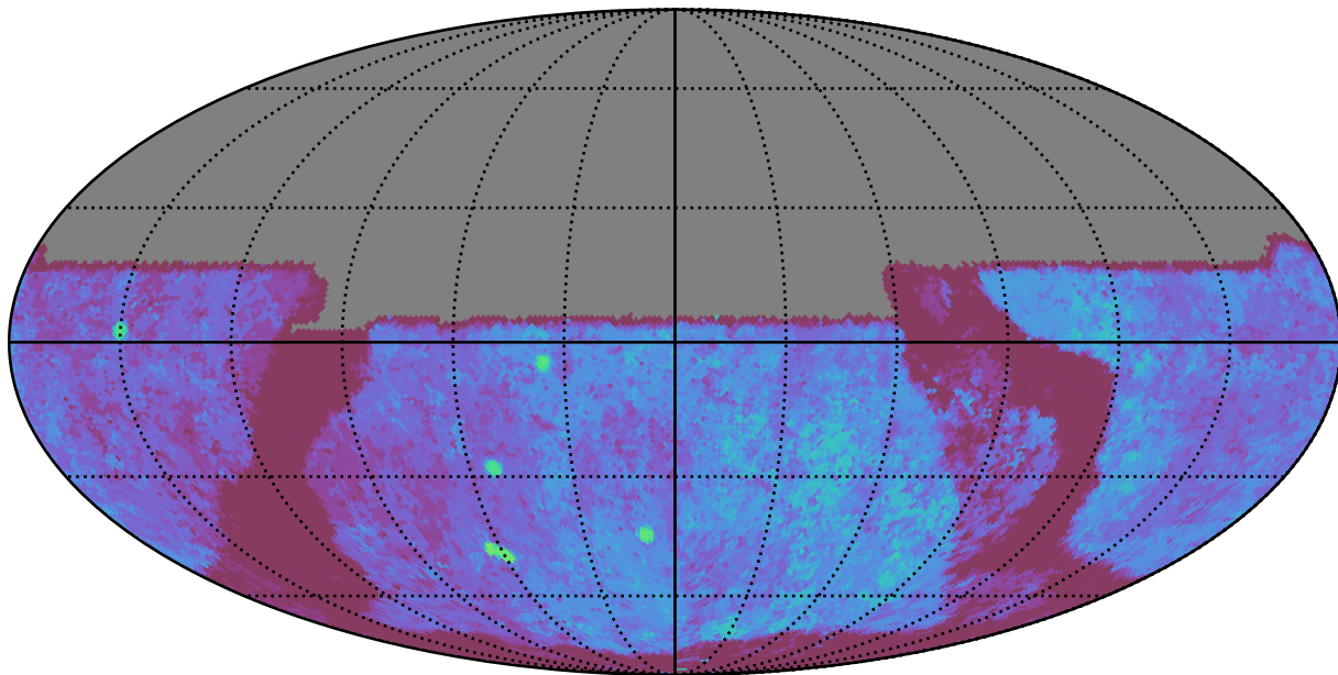
noroll_mjdp270_v3.4_10yrs All sky u band: Median Season Length
