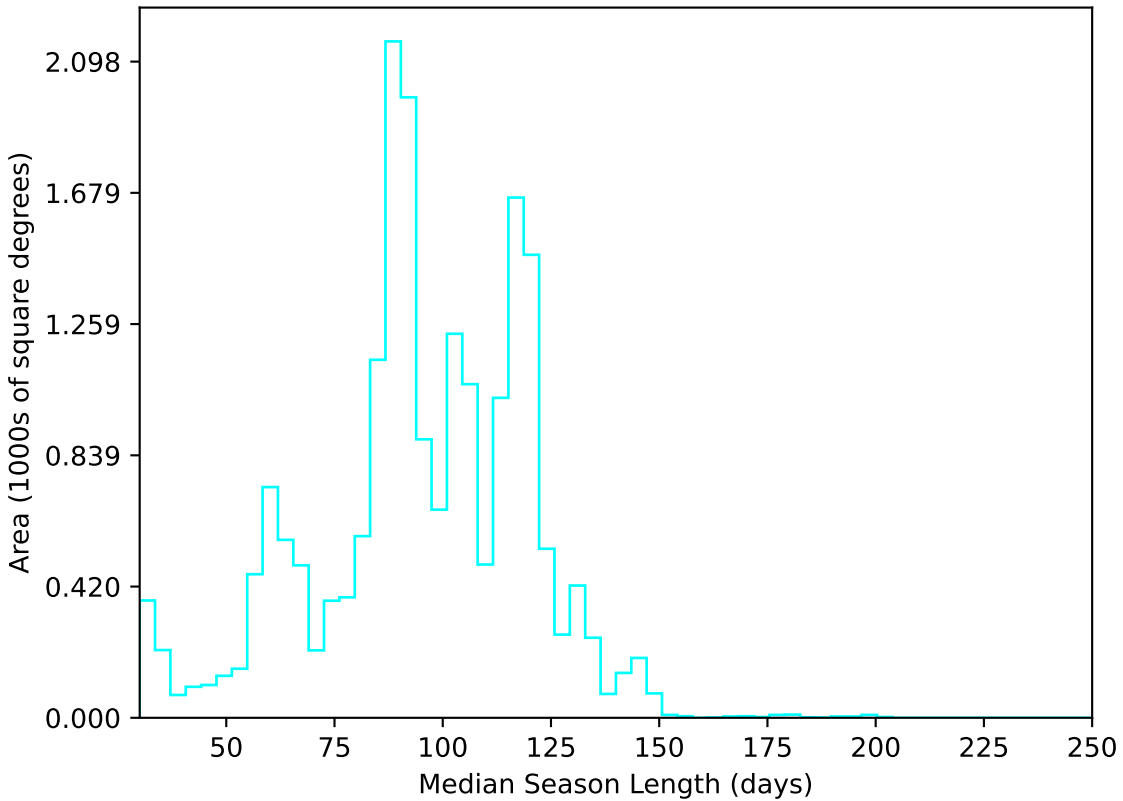
noroll_mjdp270_v3.4_10yrs All sky u band: Median Season Length
