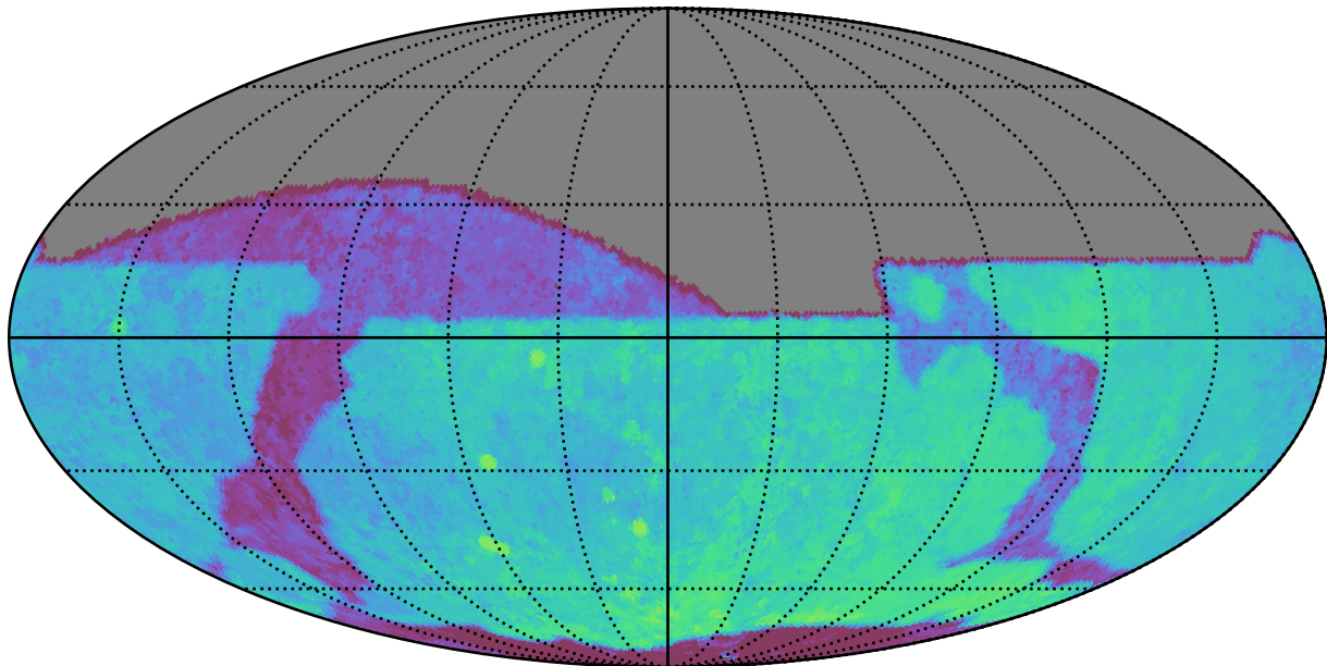
noroll_mjdp270_v3.4_10yrs All sky r band: Median Season Length
