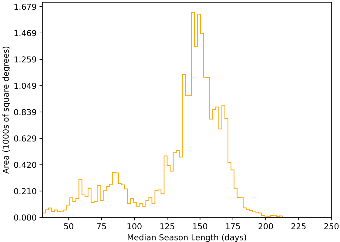
noroll_mjdp270_v3.4_10yrs All sky r band: Median Season Length
