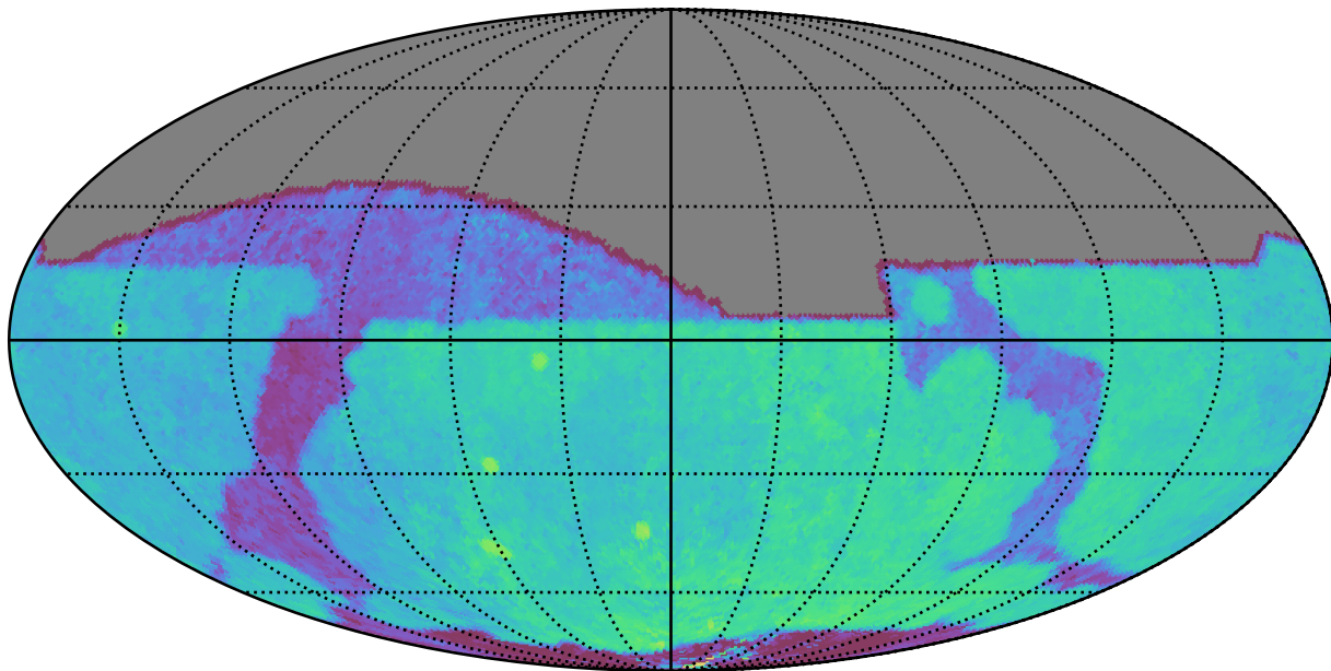
noroll_mjdp270_v3.4_10yrs All sky i band: Median Season Length
