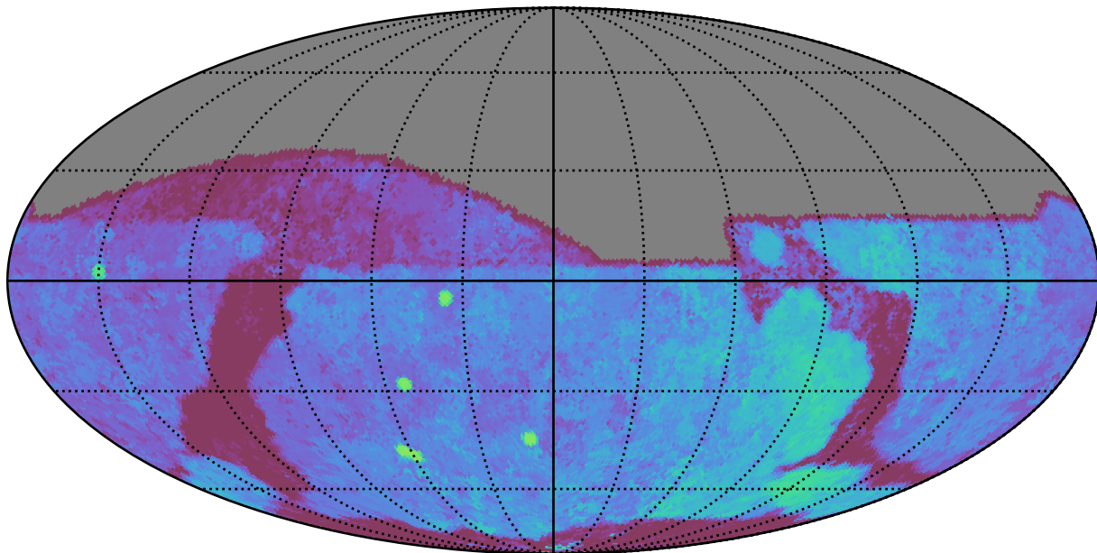
noroll_mjdp270_v3.4_10yrs All sky g band: Median Season Length
