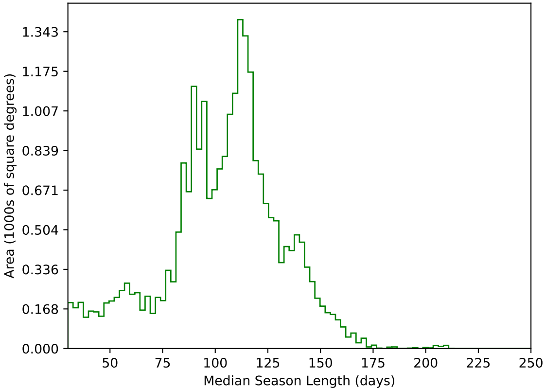
noroll_mjdp270_v3.4_10yrs All sky g band: Median Season Length
