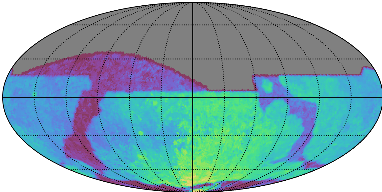
noroll_mjdp270_v3.4_10yrs All sky all bands: Median Season Length
