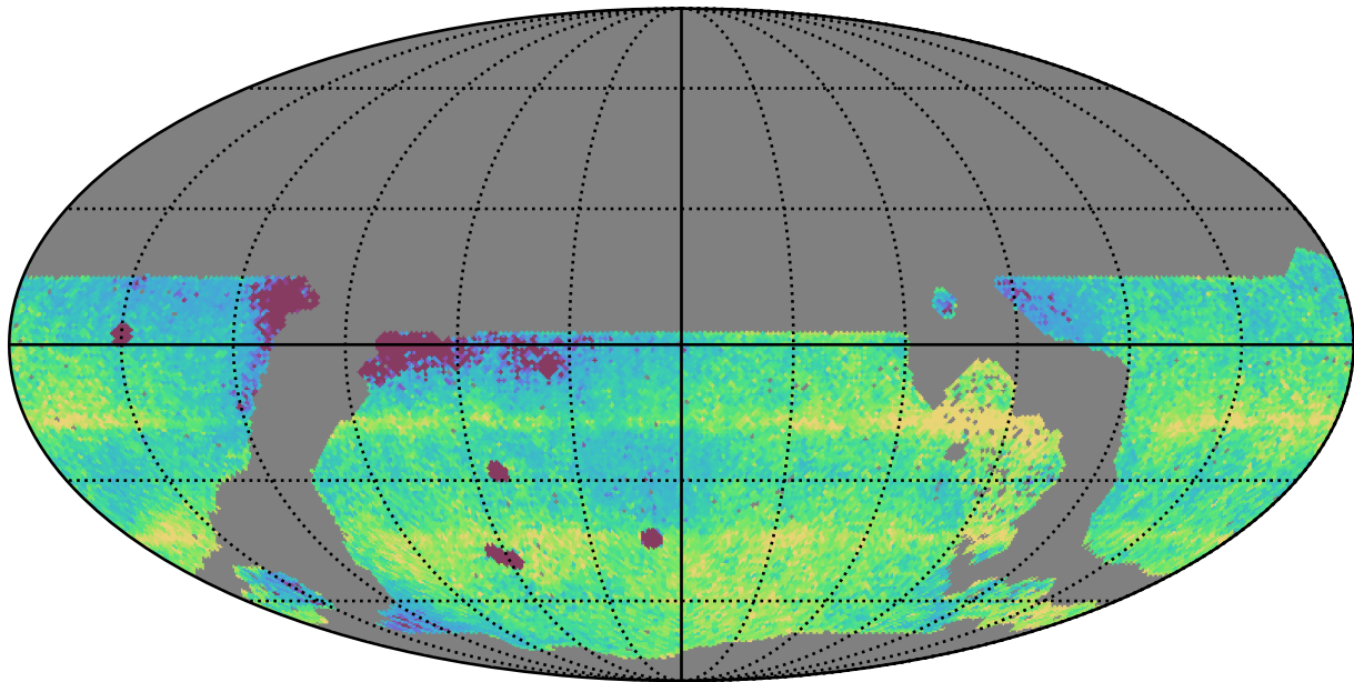
noroll_mjdp270_v3.4_10yrs WFD: Median Intra-Night Gap
