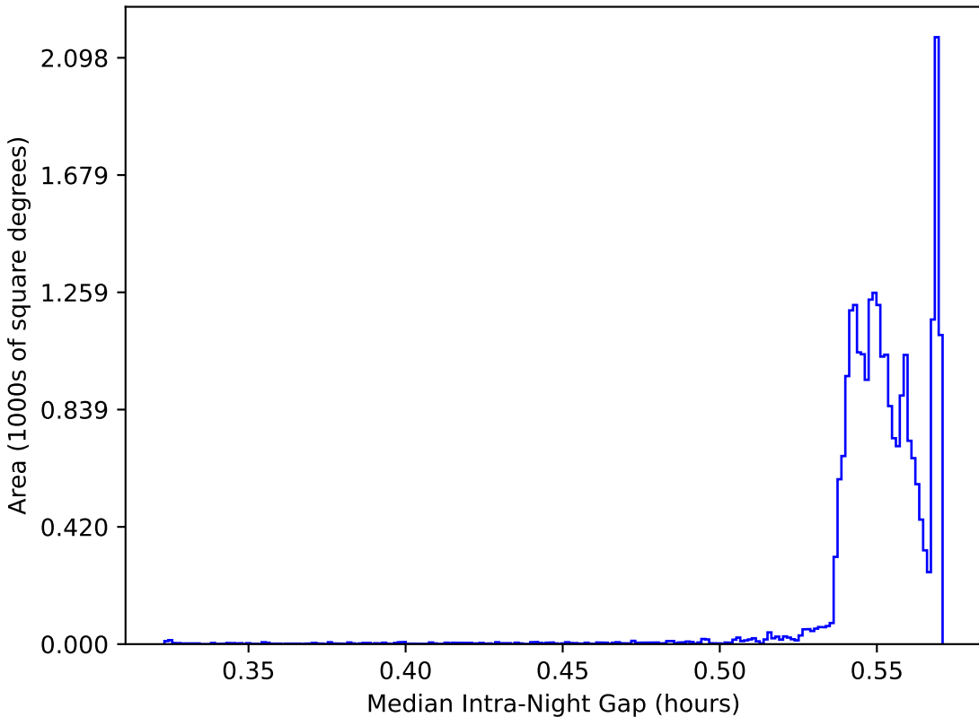
noroll_mjdp270_v3.4_10yrs All sky: Median Intra-Night Gap
