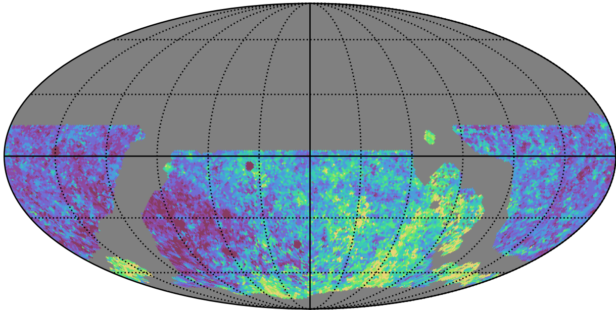
noroll_mjdp270_v3.4_10yrs WFD z band: Median Inter-Night Gap
