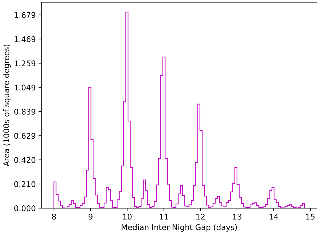
noroll_mjdp270_v3.4_10yrs WFD z band: Median Inter-Night Gap
