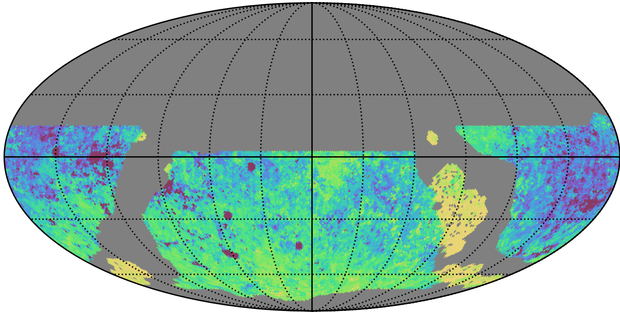
noroll_mjdp270_v3.4_10yrs WFD y band: Median Inter-Night Gap
