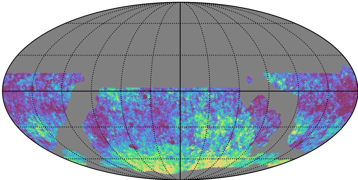
noroll_mjdp270_v3.4_10yrs WFD r band: Median Inter-Night Gap
