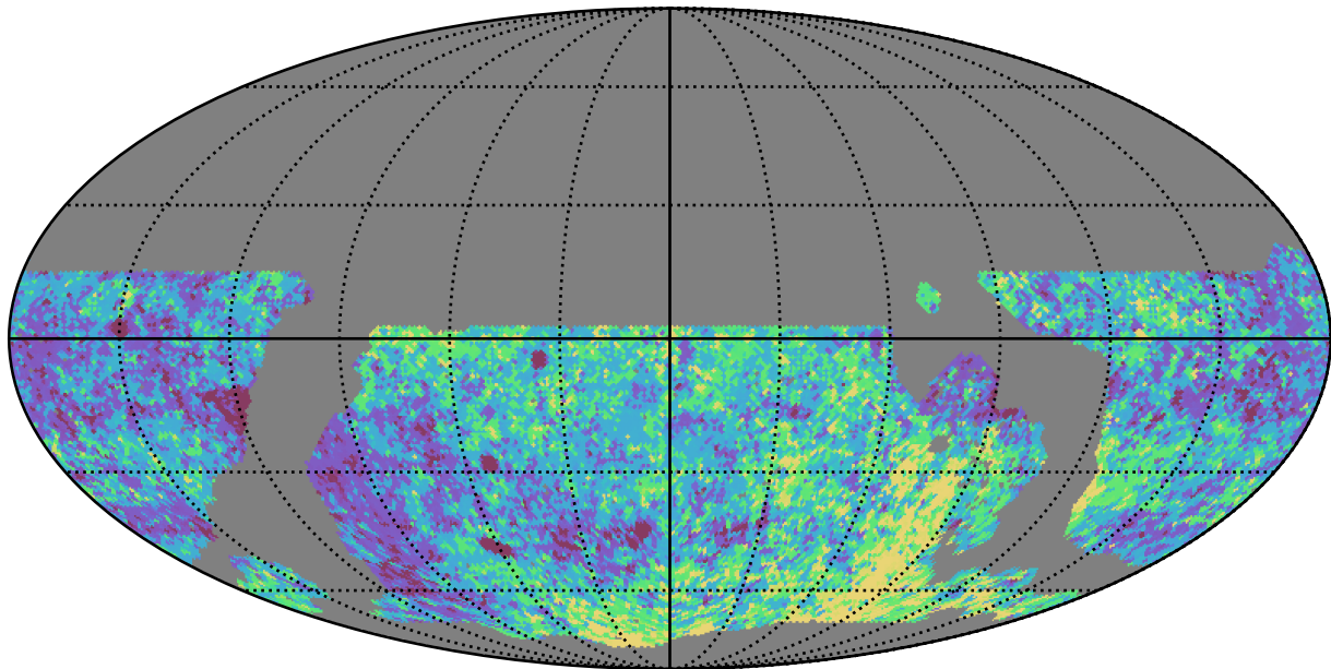
noroll_mjdp270_v3.4_10yrs WFD i band: Median Inter-Night Gap
