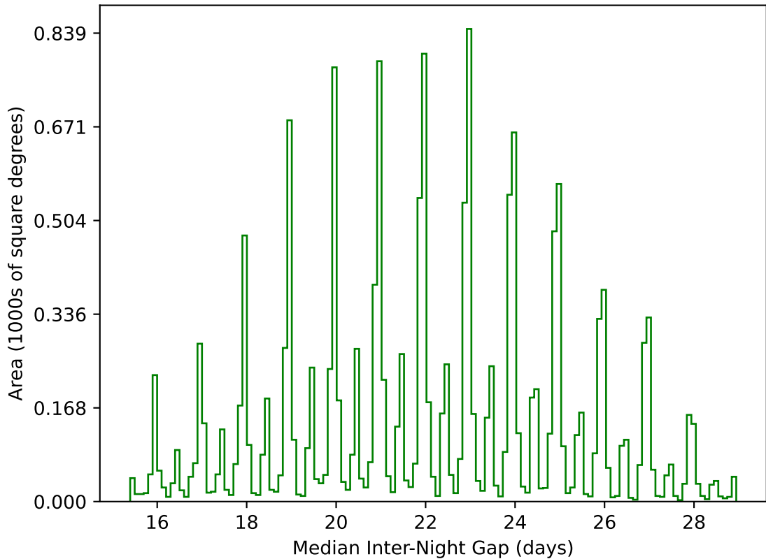
noroll_mjdp270_v3.4_10yrs WFD g band: Median Inter-Night Gap
