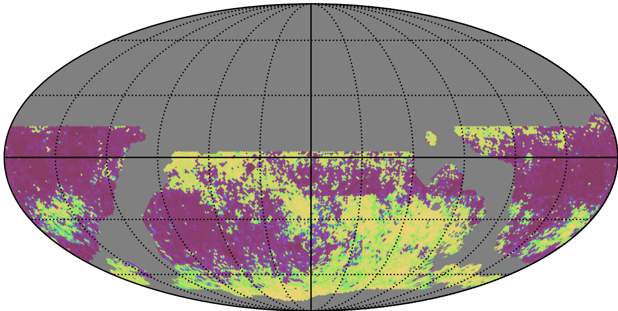
noroll_mjdp270_v3.4_10yrs WFD all bands: Median Inter-Night Gap
