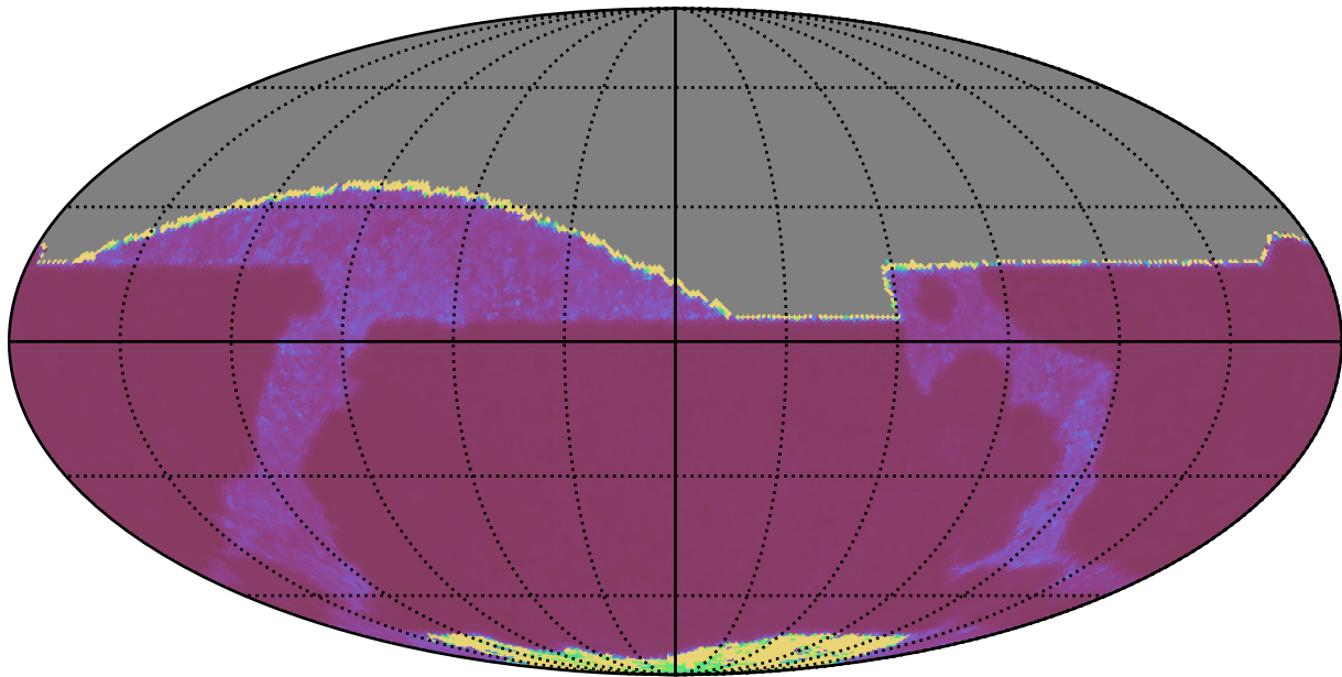
noroll_mjdp270_v3.4_10yrs All sky z band: Median Inter-Night Gap
