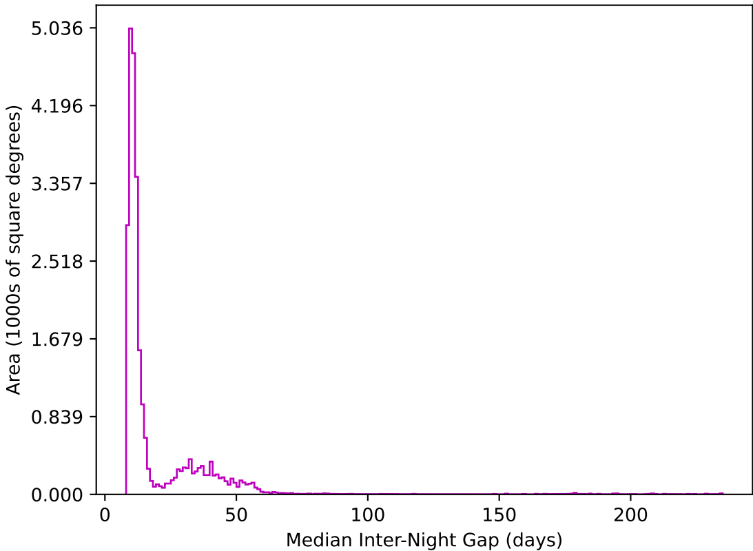
noroll_mjdp270_v3.4_10yrs All sky z band: Median Inter-Night Gap
