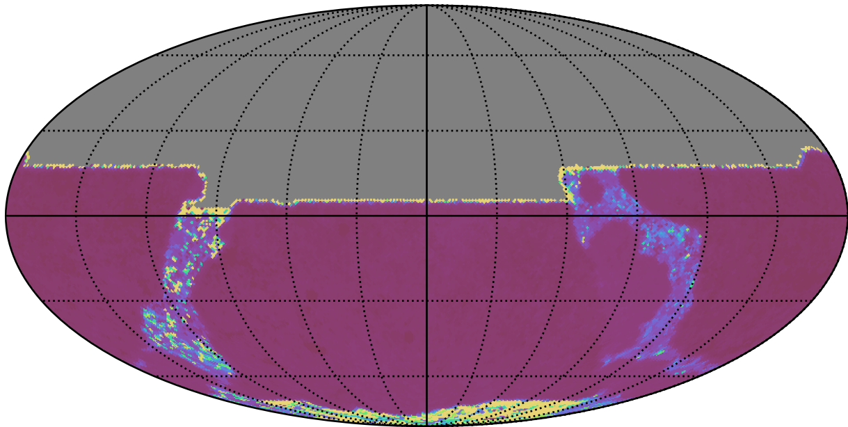
noroll_mjdp270_v3.4_10yrs All sky y band: Median Inter-Night Gap
