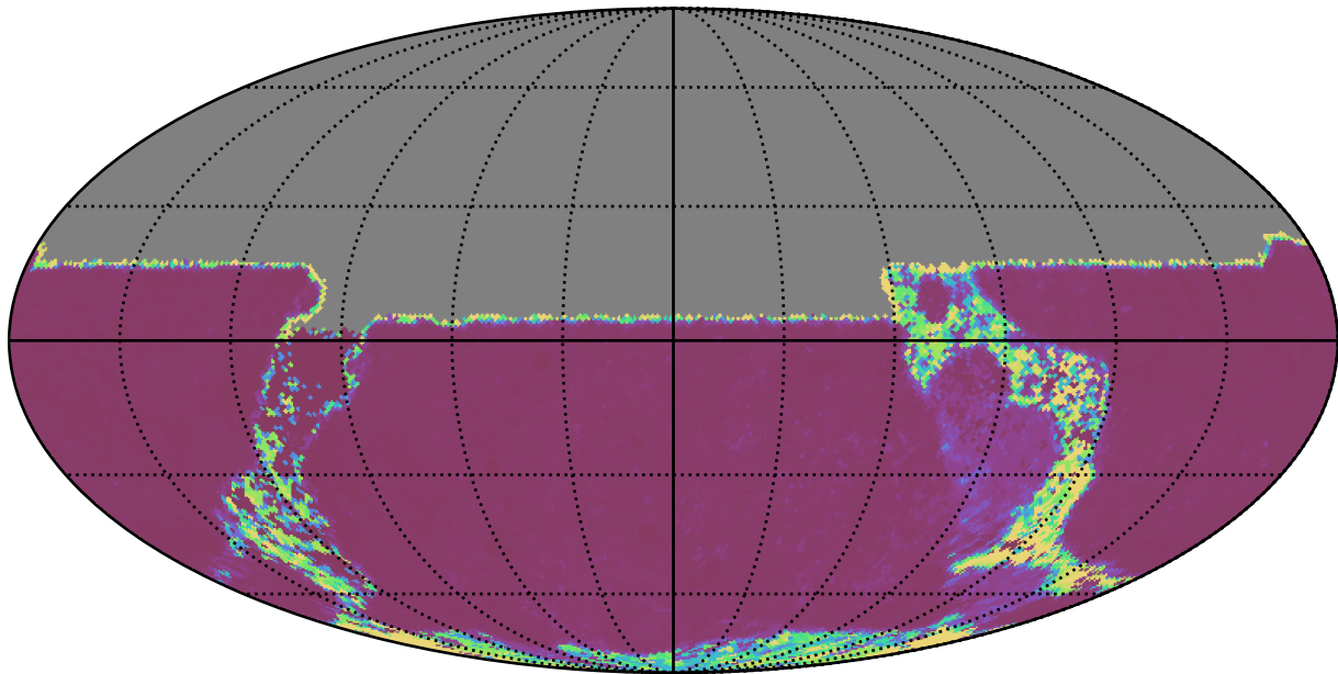
noroll_mjdp270_v3.4_10yrs All sky u band: Median Inter-Night Gap
