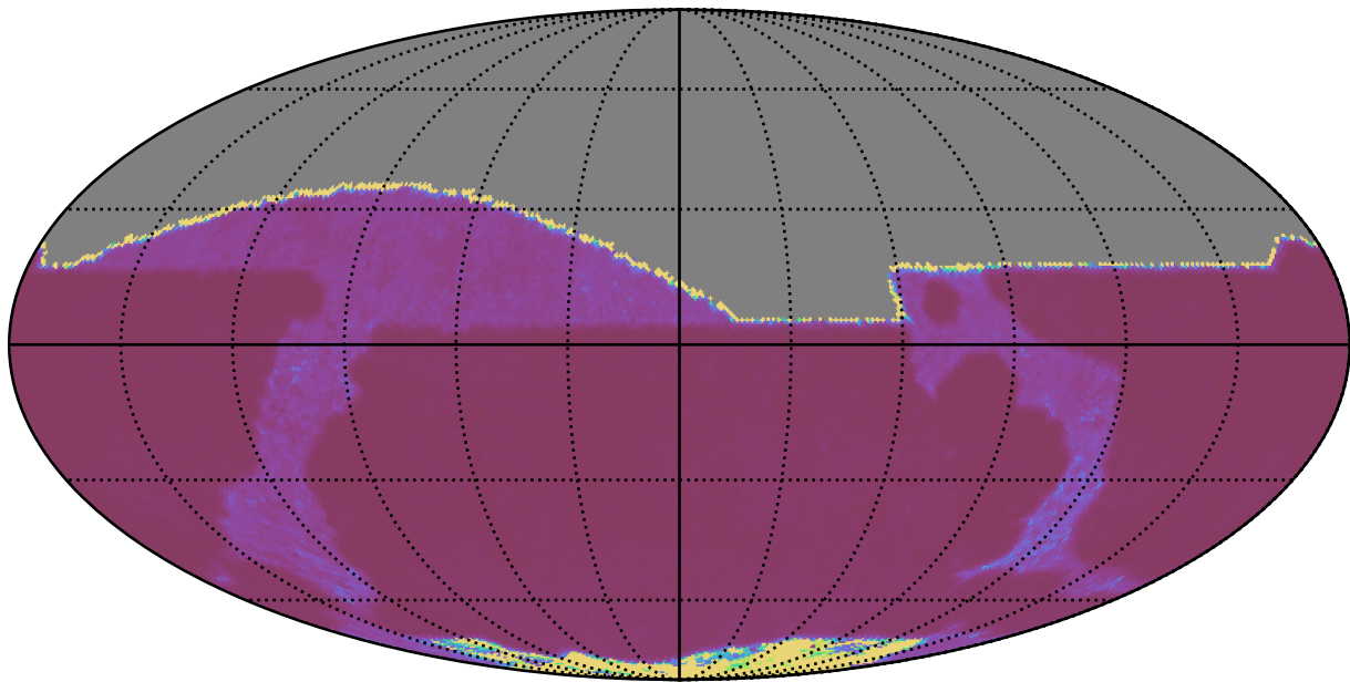
noroll_mjdp270_v3.4_10yrs All sky r band: Median Inter-Night Gap
