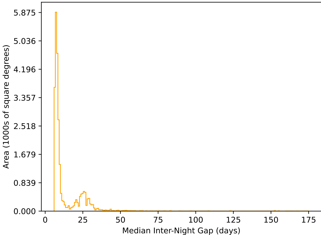
noroll_mjdp270_v3.4_10yrs All sky r band: Median Inter-Night Gap
