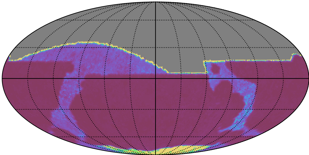
noroll_mjdp270_v3.4_10yrs All sky i band: Median Inter-Night Gap
