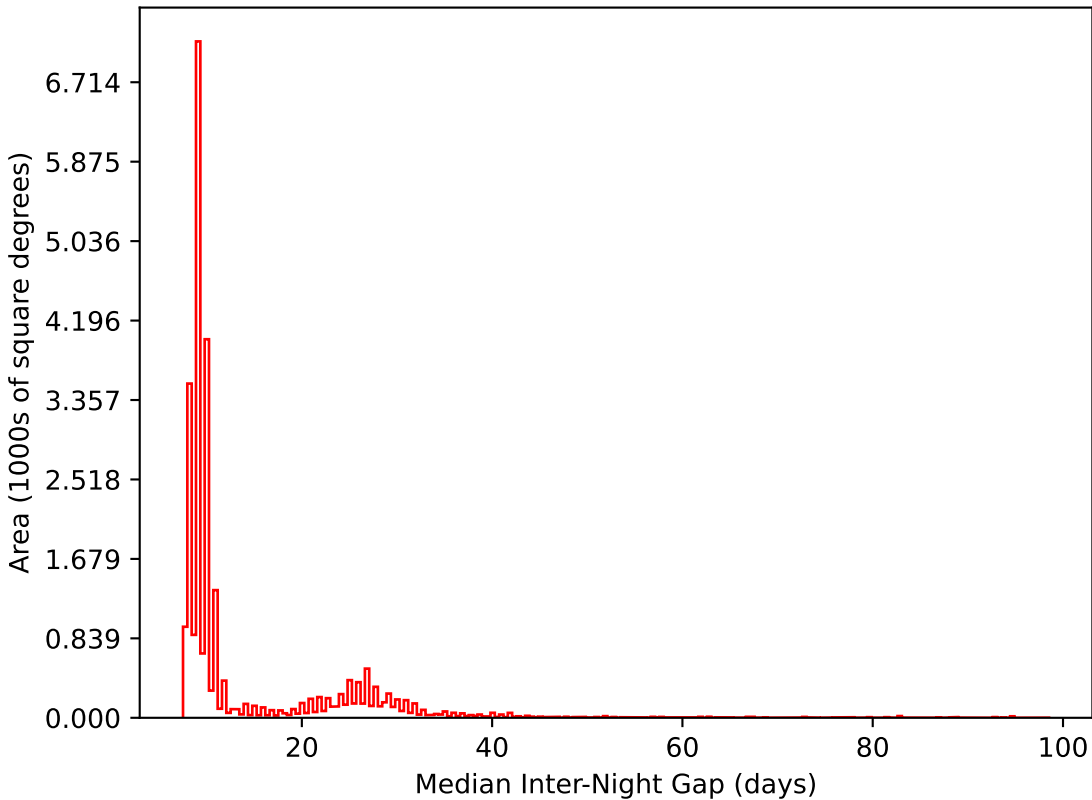
noroll_mjdp270_v3.4_10yrs All sky i band: Median Inter-Night Gap
