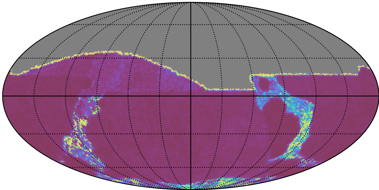
noroll_mjdp270_v3.4_10yrs All sky g band: Median Inter-Night Gap
