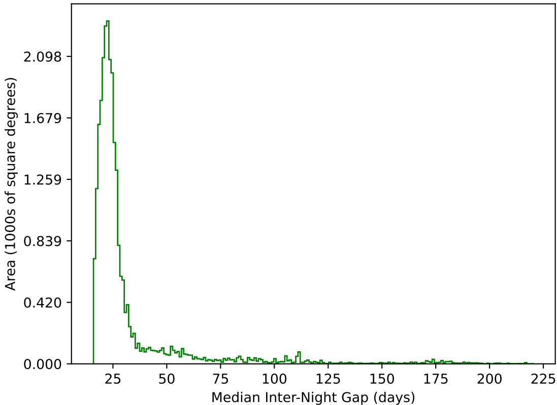
noroll_mjdp270_v3.4_10yrs All sky g band: Median Inter-Night Gap
