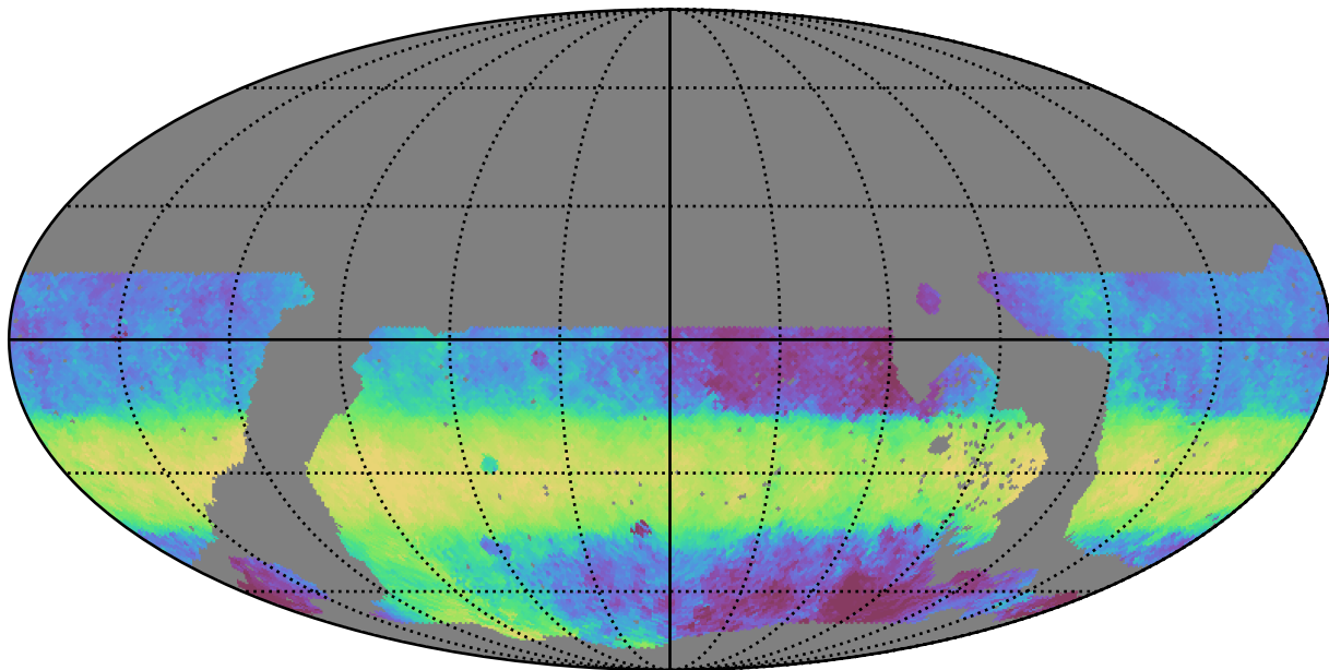
noroll_mjdp270_v3.4_10yrs WFD y band: Median HA
