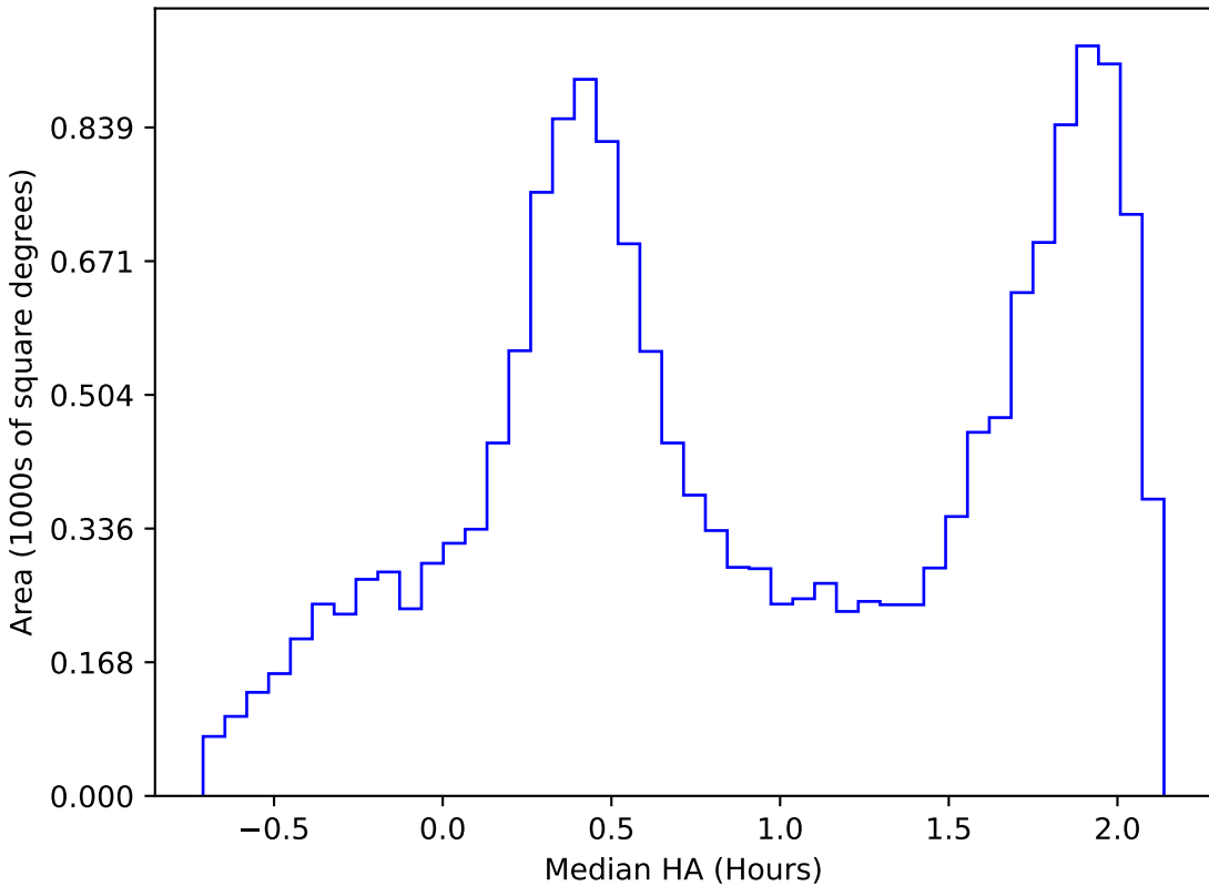
noroll_mjdp270_v3.4_10yrs WFD y band: Median HA
