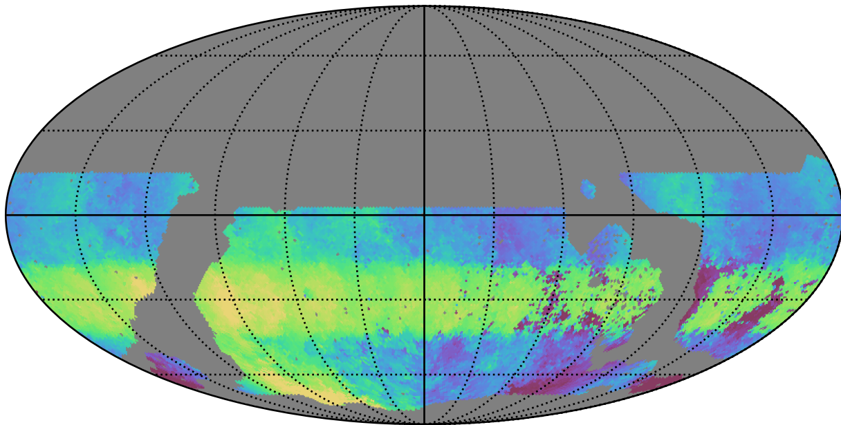
noroll_mjdp270_v3.4_10yrs WFD u band: Median HA
