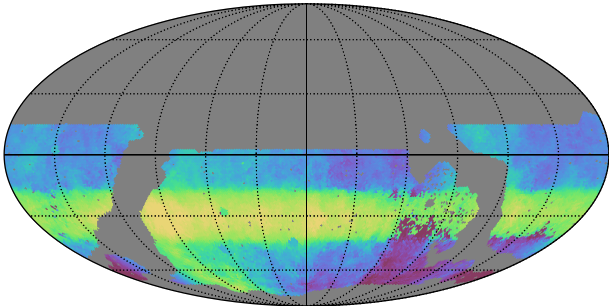
noroll_mjdp270_v3.4_10yrs WFD r band: Median HA
