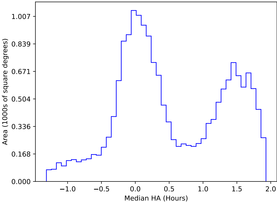
noroll_mjdp270_v3.4_10yrs WFD r band: Median HA
