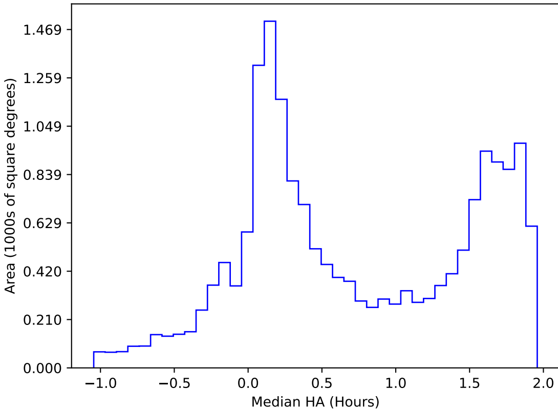
noroll_mjdp270_v3.4_10yrs WFD all bands: Median HA
