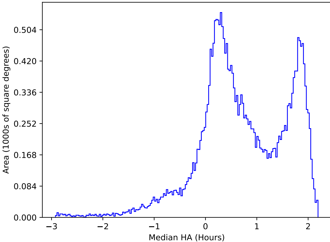
noroll_mjdp270_v3.4_10yrs All sky z band: Median HA
