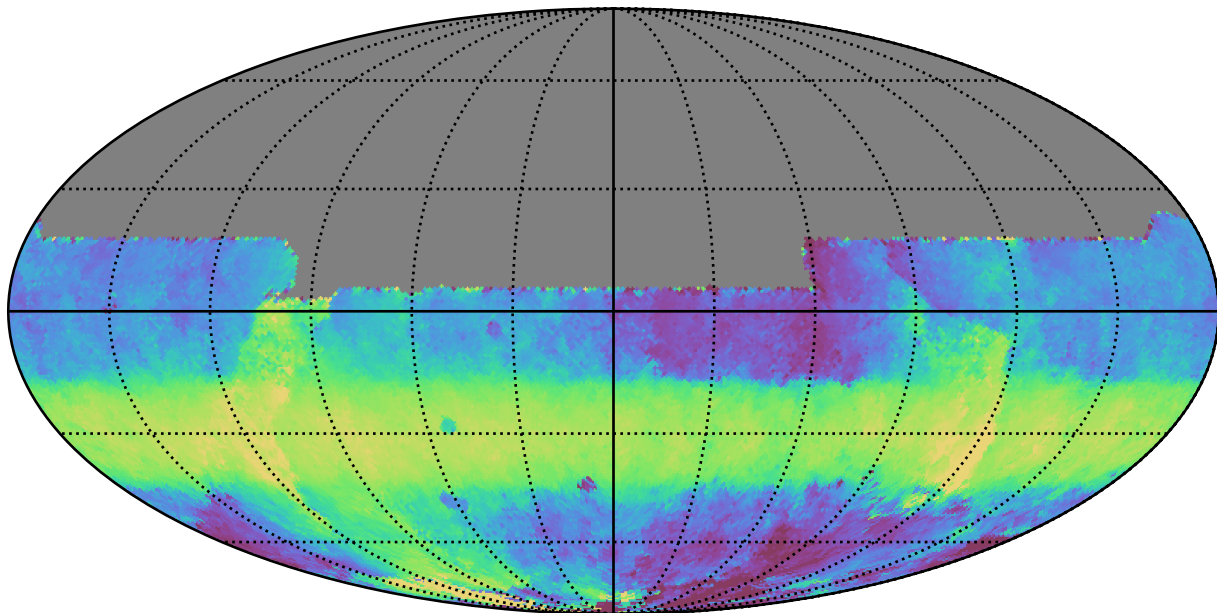
noroll_mjdp270_v3.4_10yrs All sky y band: Median HA
