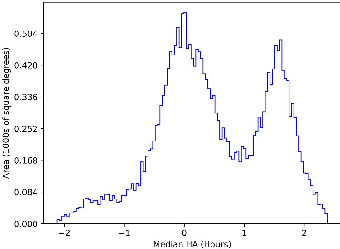
noroll_mjdp270_v3.4_10yrs All sky u band: Median HA
