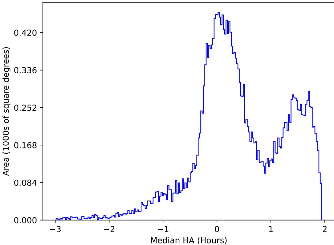
noroll_mjdp270_v3.4_10yrs All sky r band: Median HA
