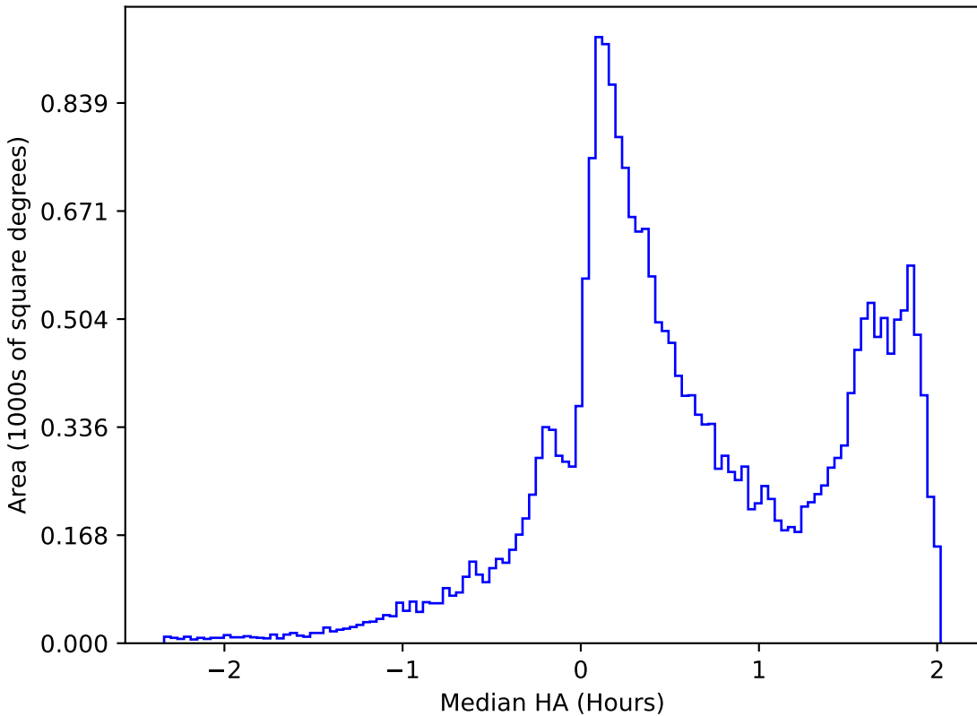
noroll_mjdp270_v3.4_10yrs All sky all bands: Median HA
