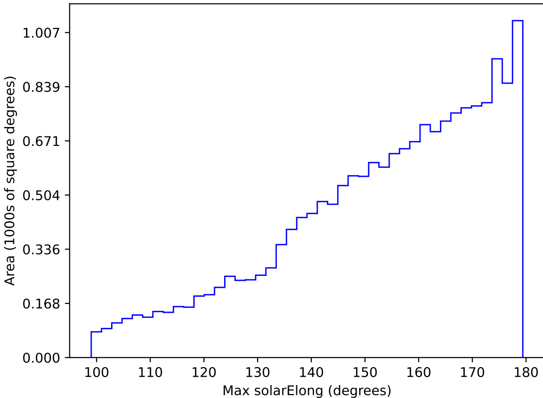
noroll_mjdp270_v3.4_10yrs WFD z band: Max solarElong
