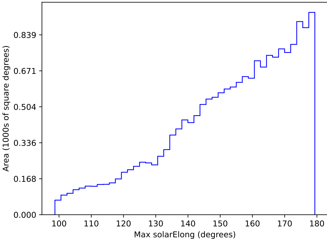
noroll_mjdp270_v3.4_10yrs WFD y band: Max solarElong
