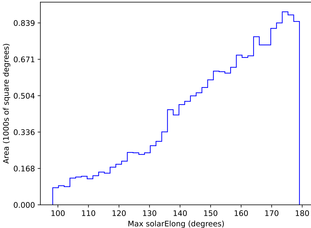
noroll_mjdp270_v3.4_10yrs WFD u band: Max solarElong
