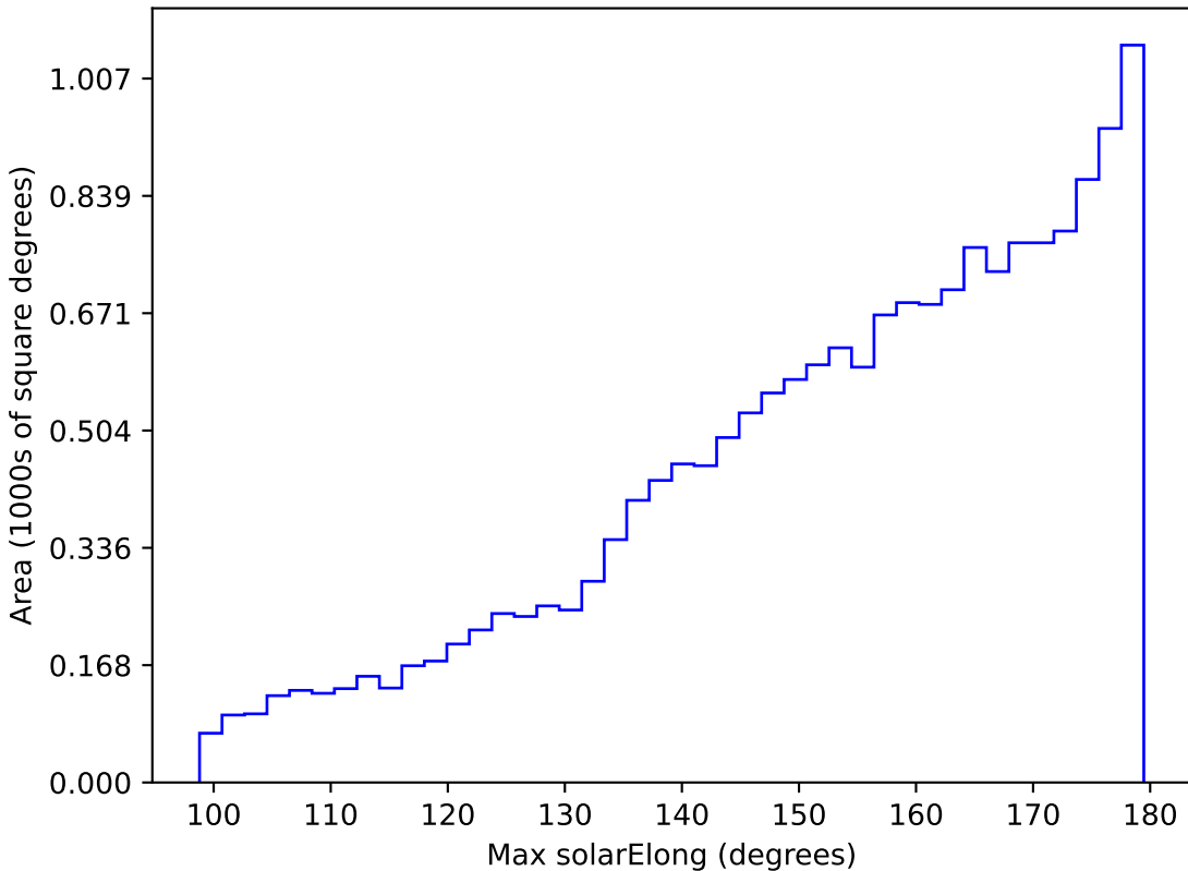
noroll_mjdp270_v3.4_10yrs WFD r band: Max solarElong
