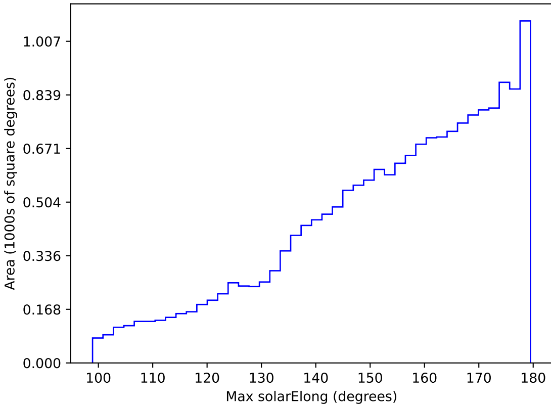
noroll_mjdp270_v3.4_10yrs WFD i band: Max solarElong
