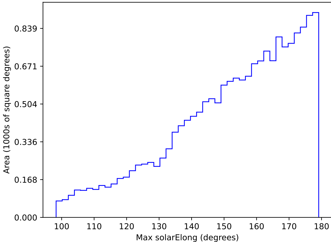
noroll_mjdp270_v3.4_10yrs WFD g band: Max solarElong
