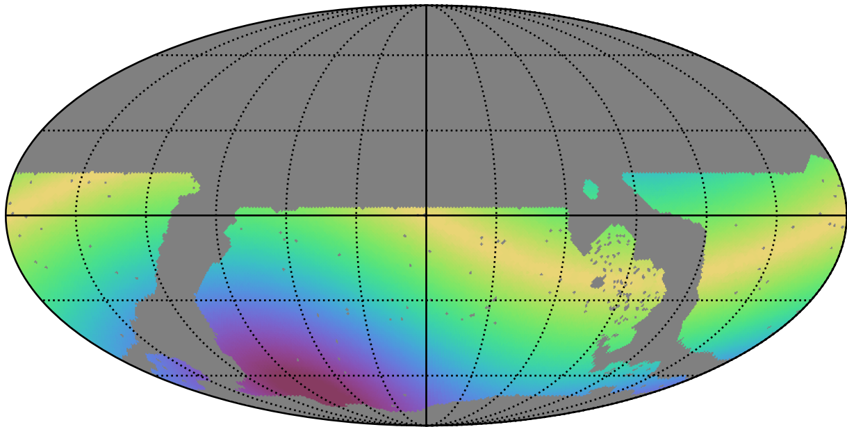
noroll_mjdp270_v3.4_10yrs WFD all bands: Max solarElong
