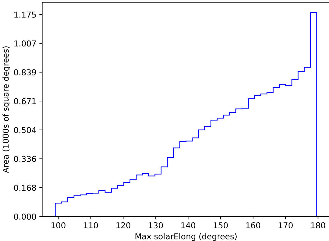
noroll_mjdp270_v3.4_10yrs WFD all bands: Max solarElong
