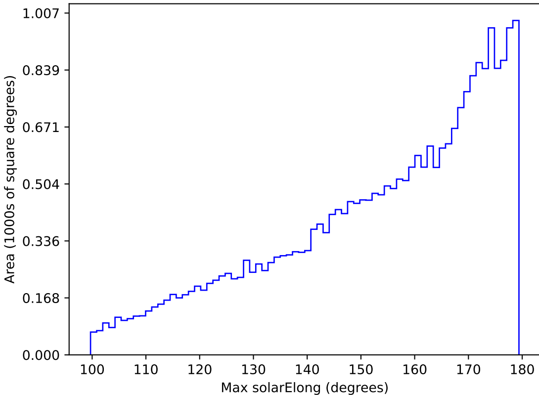
noroll_mjdp270_v3.4_10yrs All sky z band: Max solarElong
