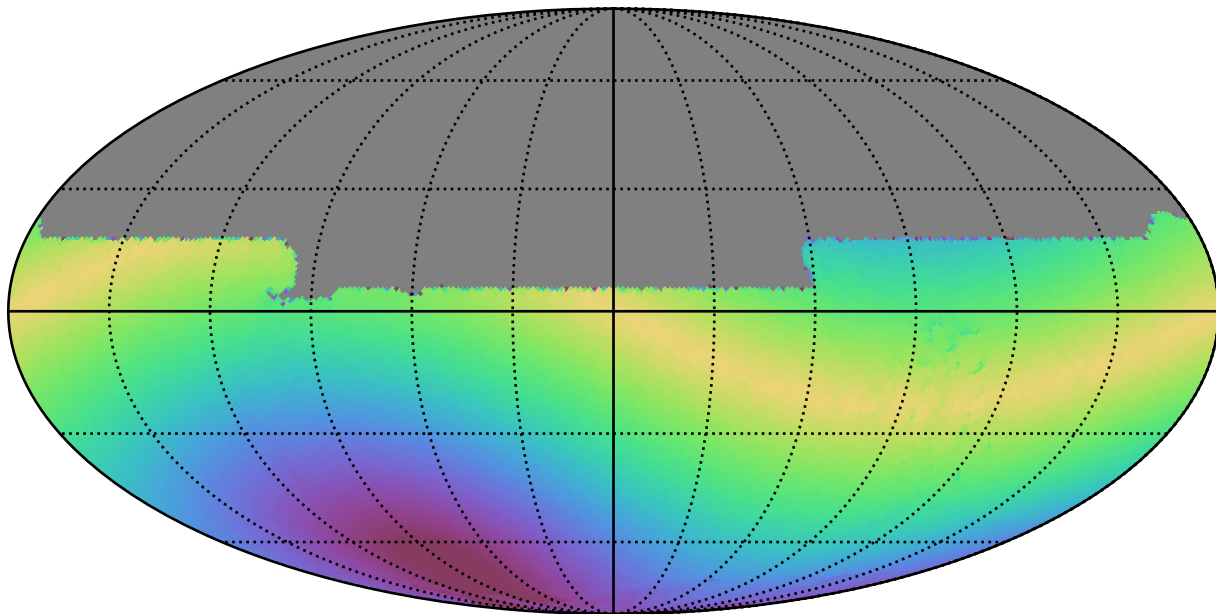
noroll_mjdp270_v3.4_10yrs All sky y band: Max solarElong
